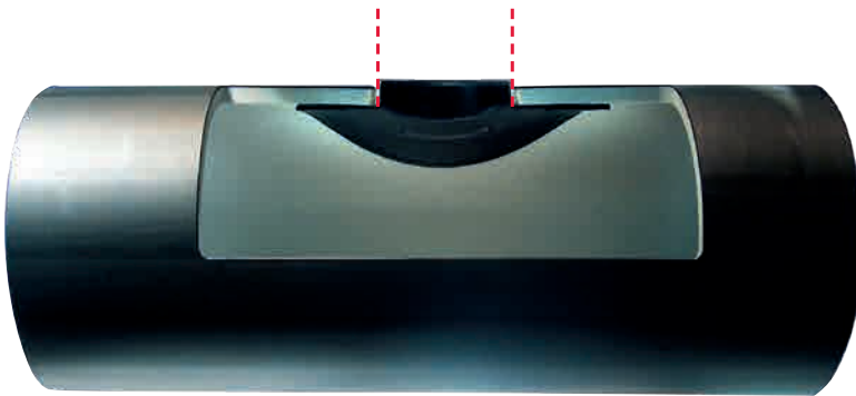
Internal saddle with transition to service connection – Felt collar for the purpose of attaching needle-felt hose as part of rehabilitation projects
